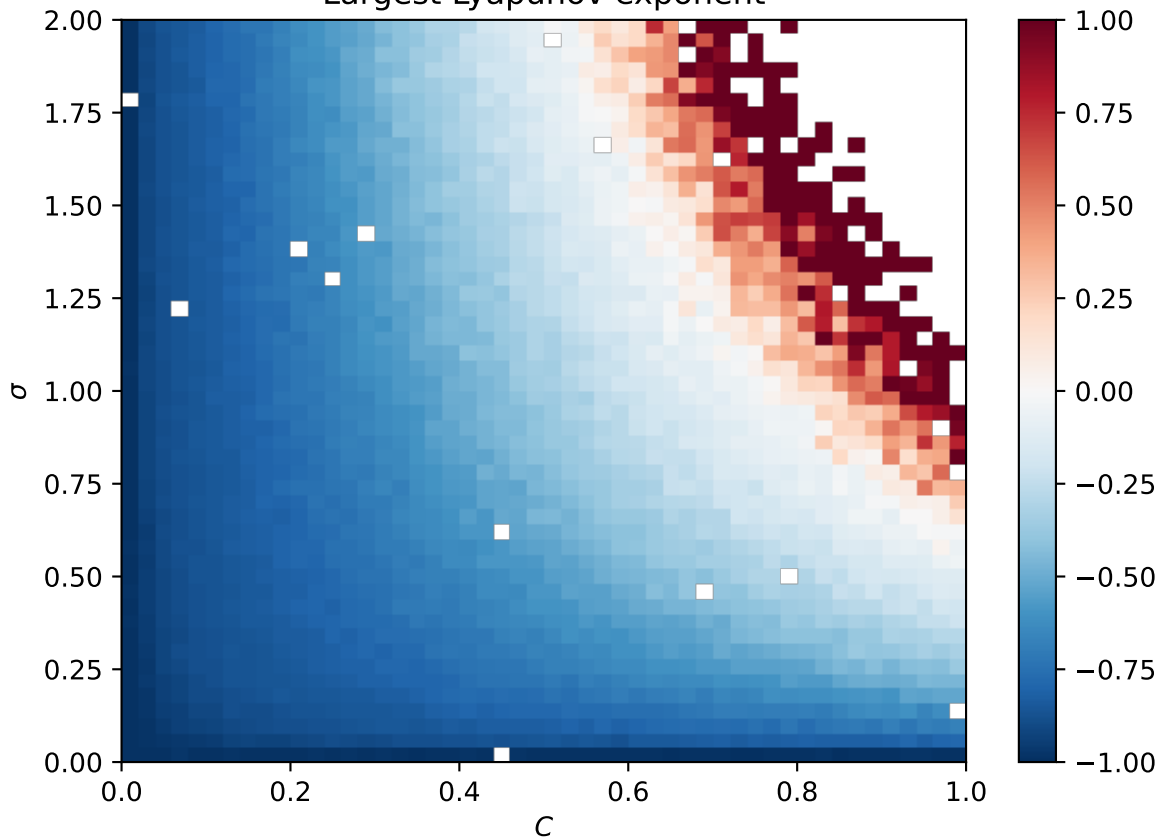
Largest Lyapunov exponent
